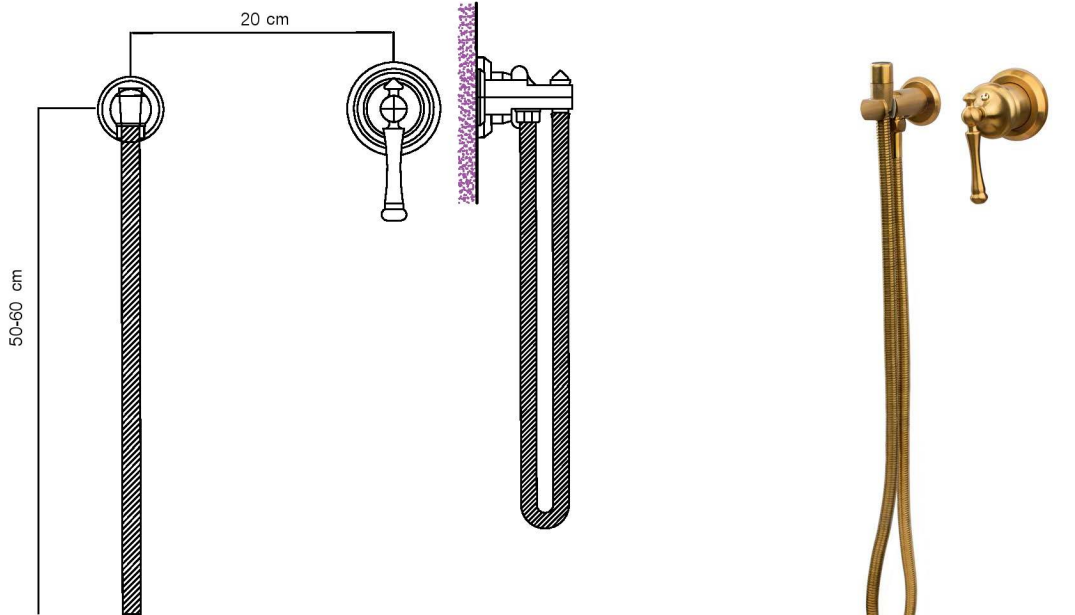
SHOWER MIXER
