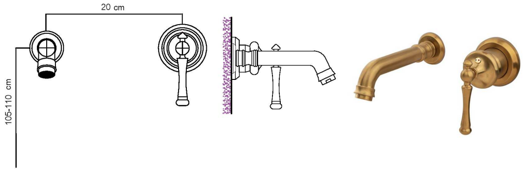
BASIN MIXER
